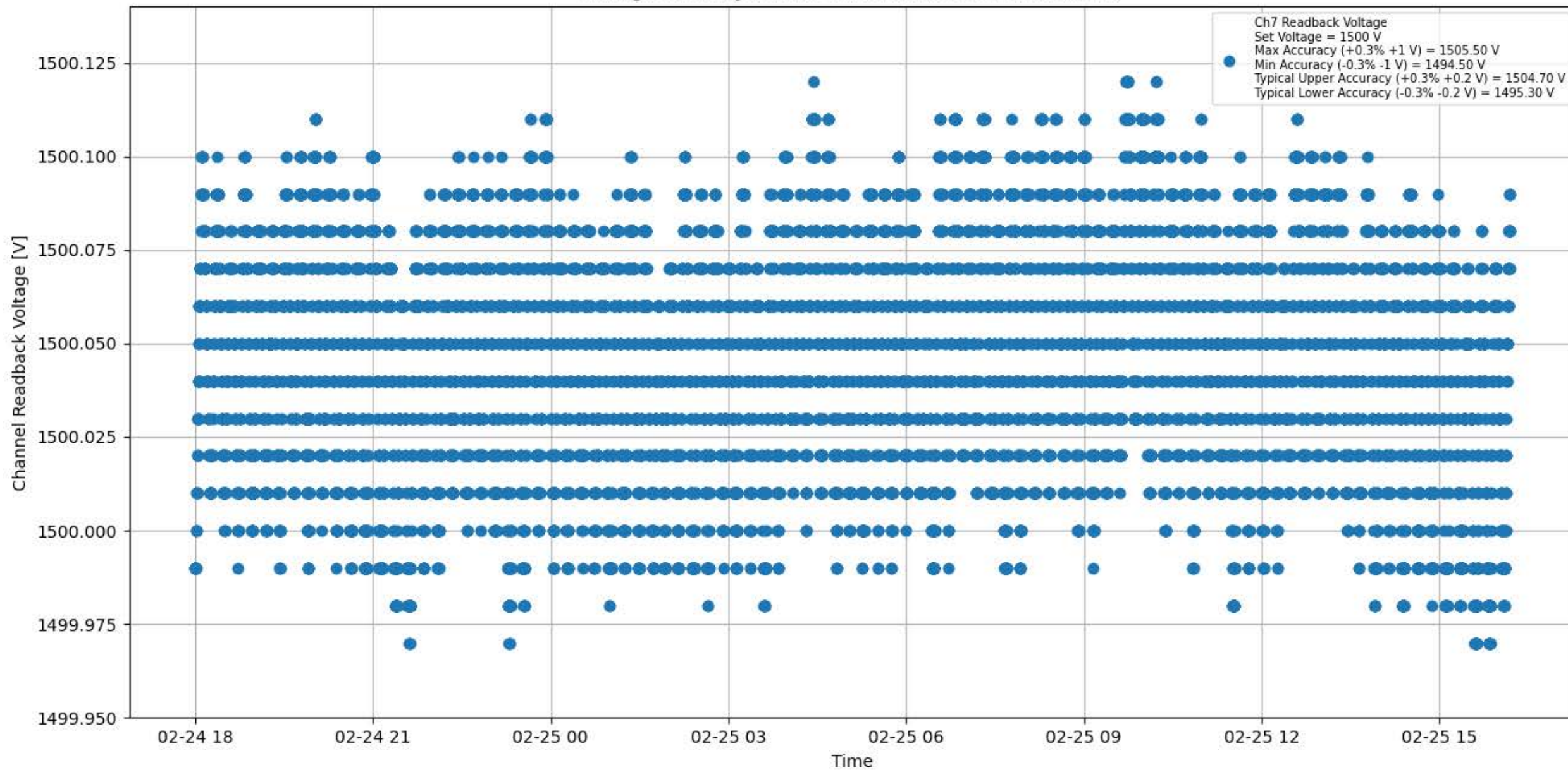
Voltage Stability 1500 V for Module #094 Channel #7
