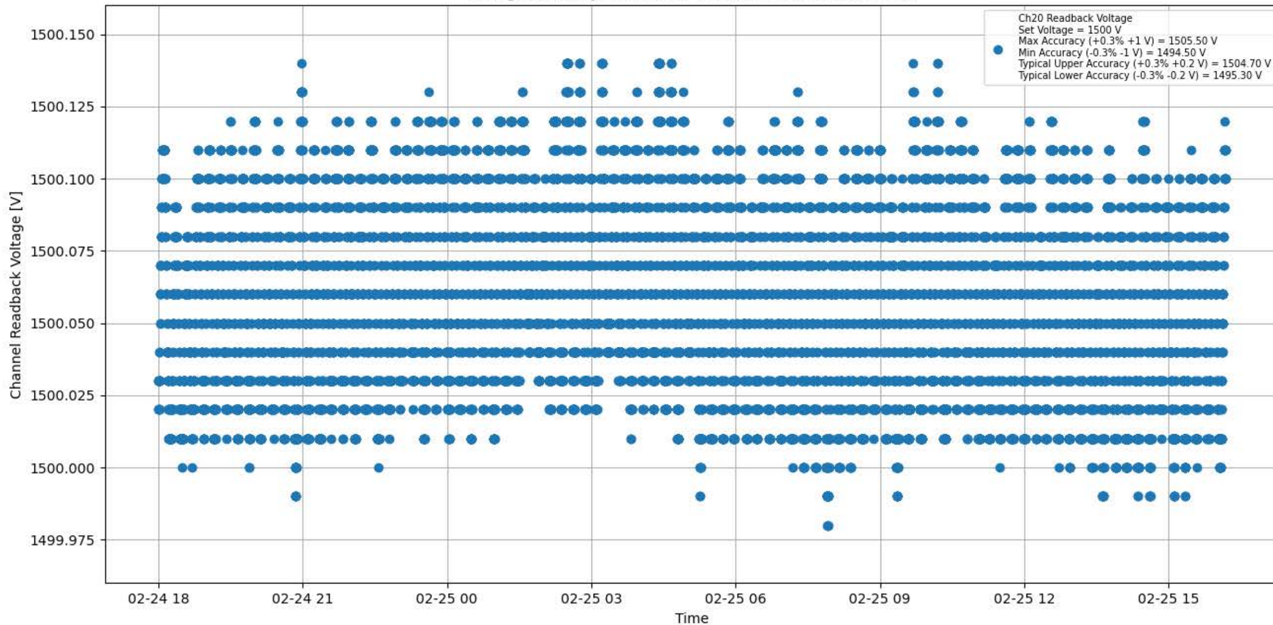
Voltage Stability 1500 V for Module #094 Channel #20
