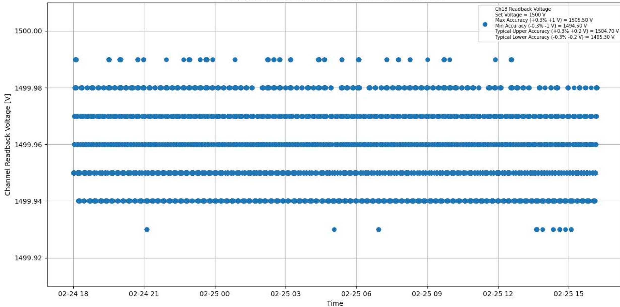
Voltage Stability 1500 V for Module #094 Channel #18
