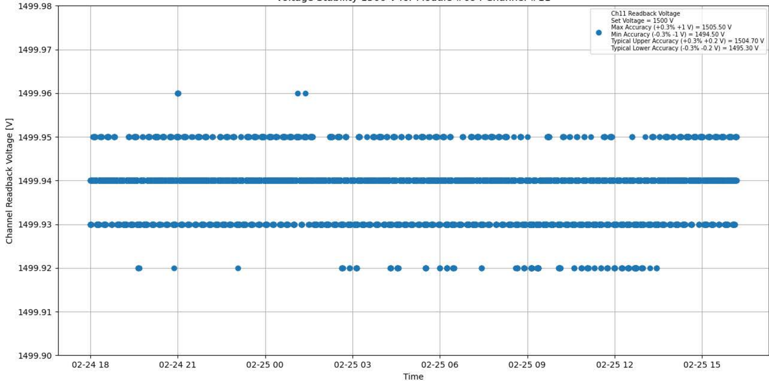
Voltage Stability 1500 V for Module #094 Channel #11
