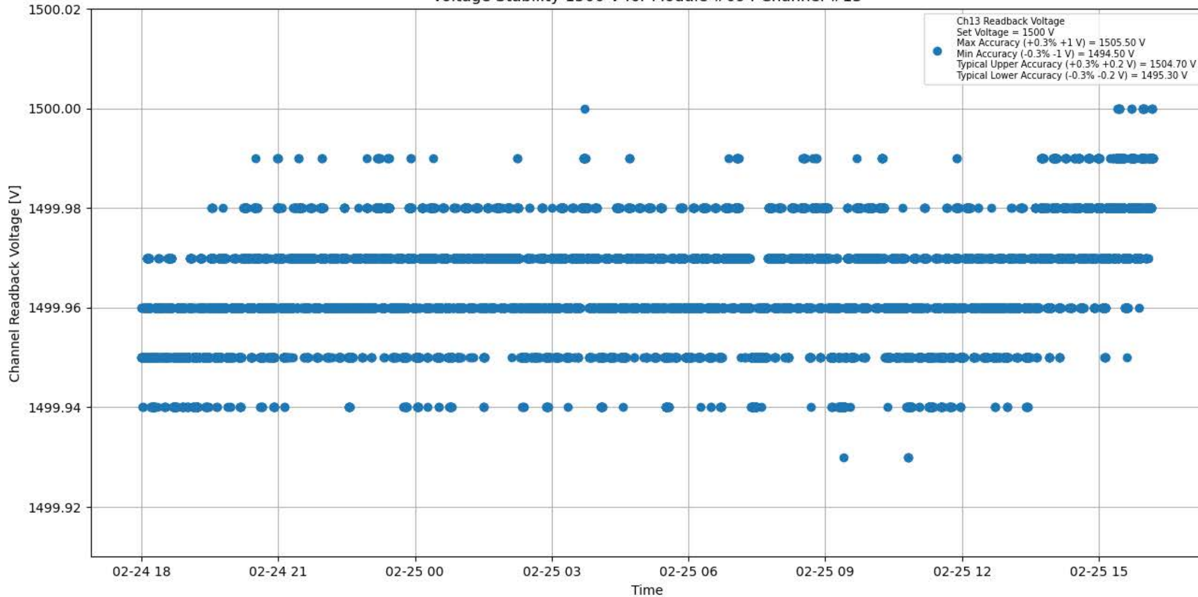
Voltage Stability 1500 V for Module #094 Channel #13
