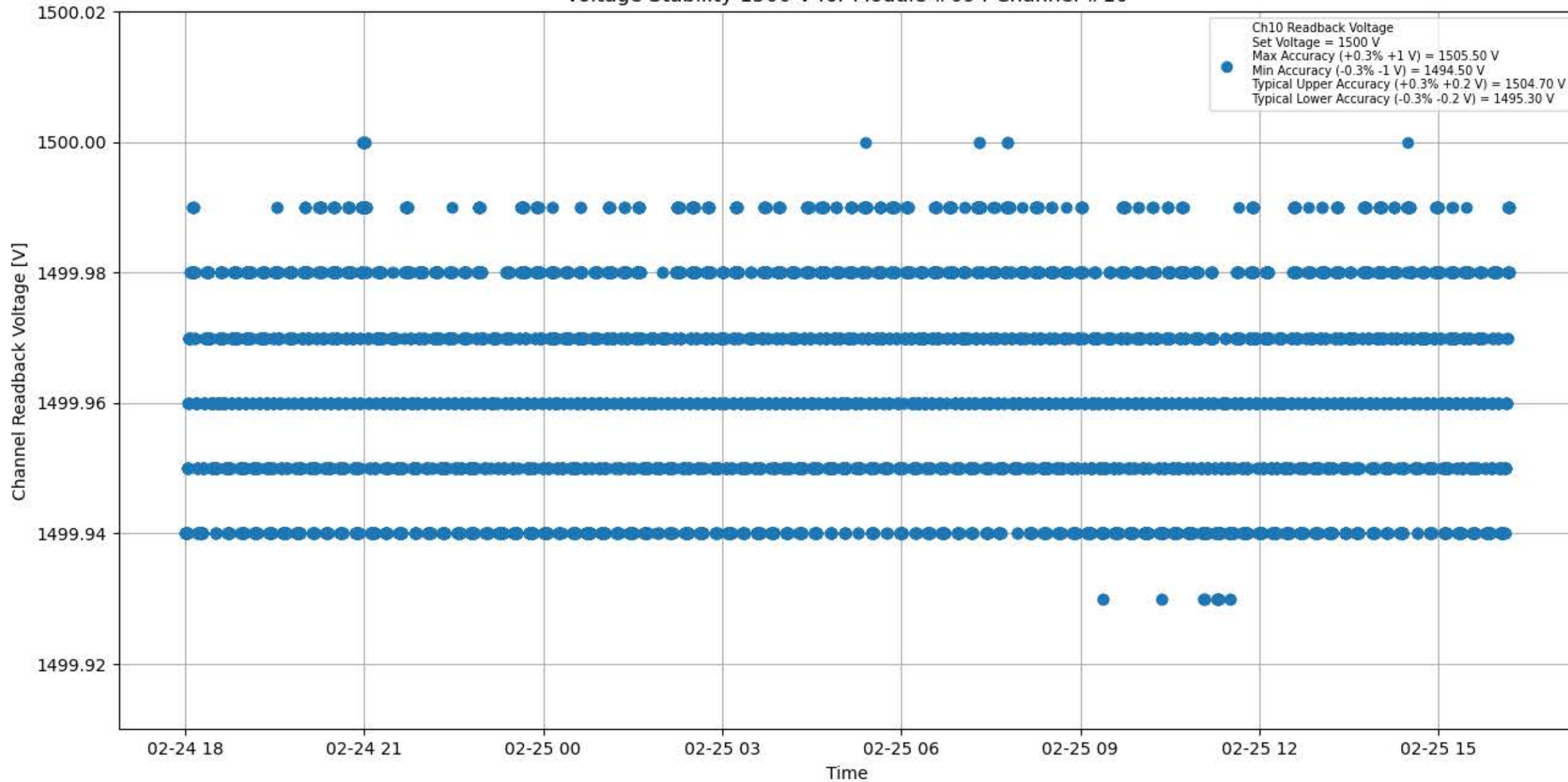
Voltage Stability 1500 V for Module #094 Channel #10
