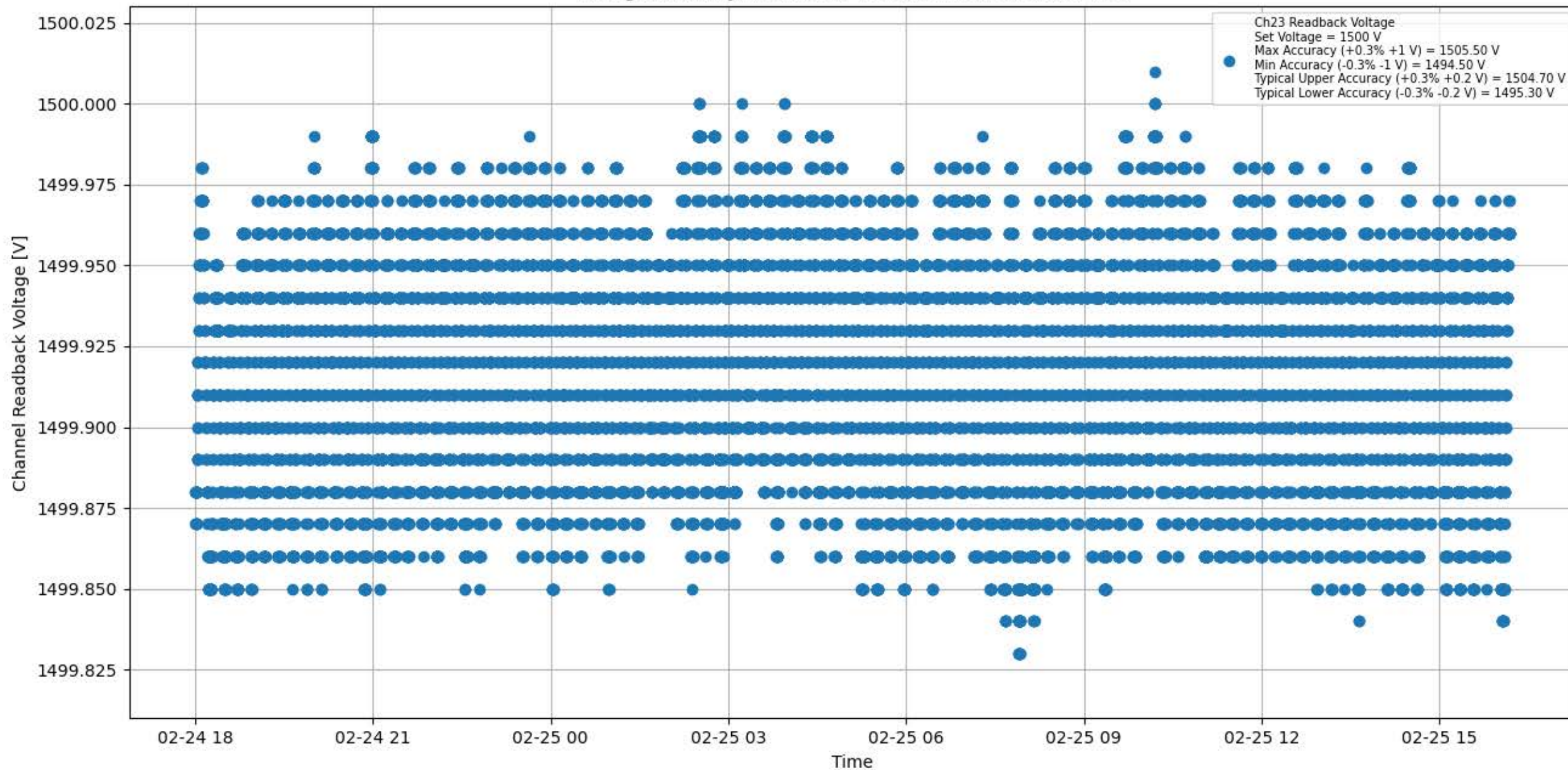
Voltage Stability 1500 V for Module #094 Channel #23
