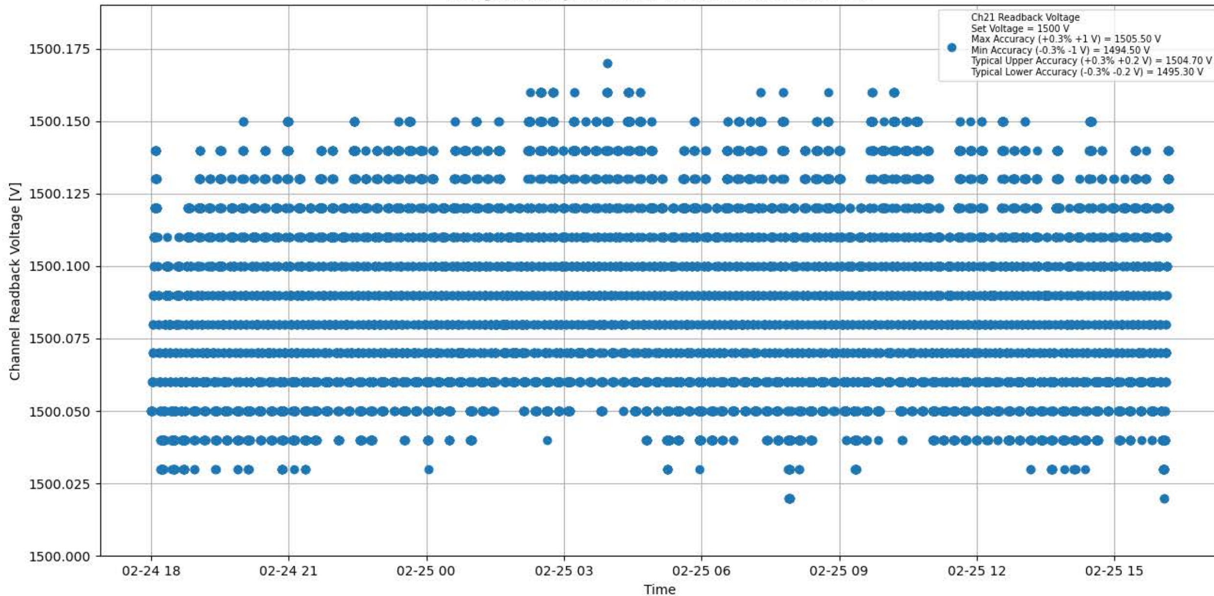
Voltage Stability 1500 V for Module #094 Channel #21
