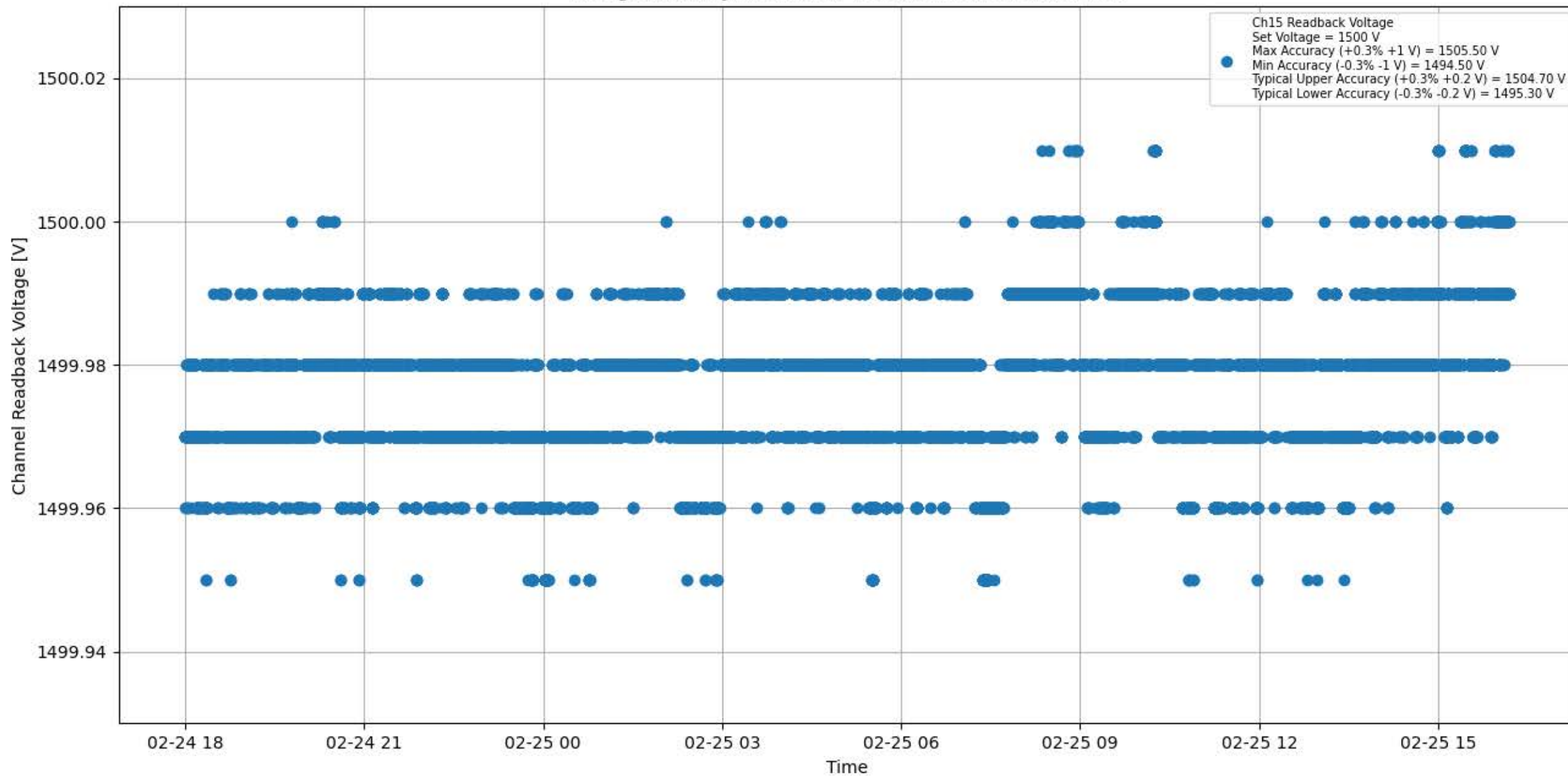
Voltage Stability 1500 V for Module #094 Channel #15
