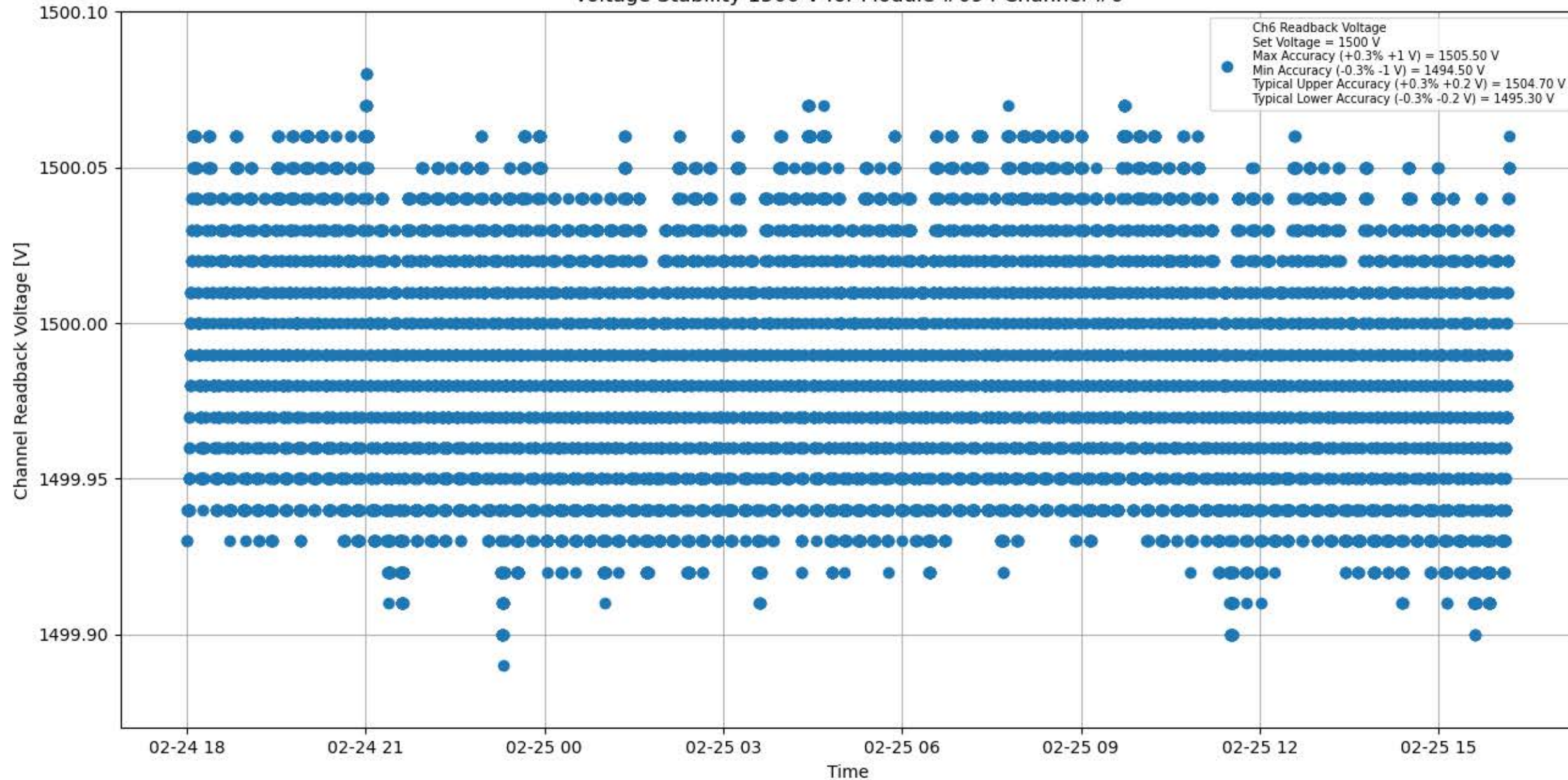
Voltage Stability 1500 V for Module #094 Channel #6
