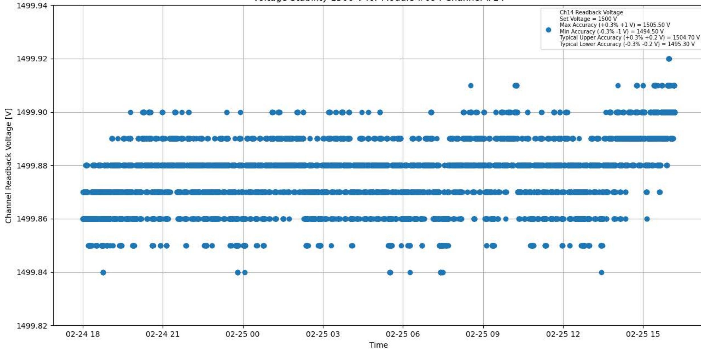
Voltage Stability 1500 V for Module #094 Channel #14
