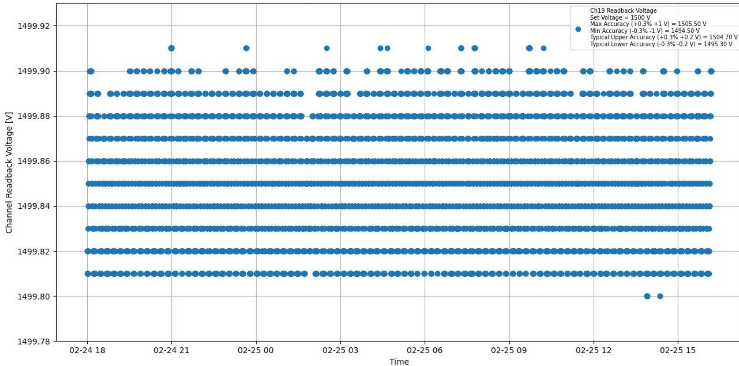
Voltage Stability 1500 V for Module #094 Channel #19
