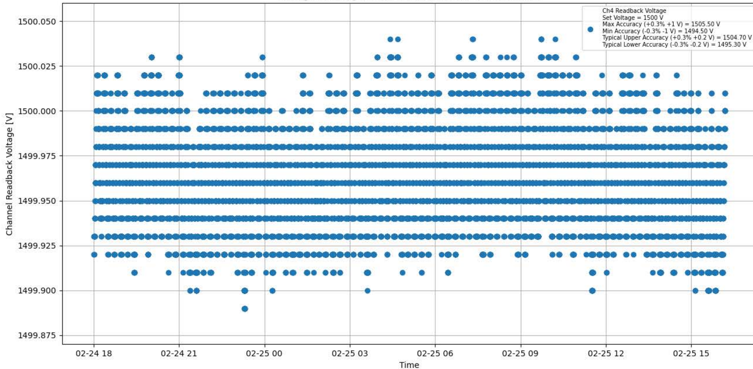
Voltage Stability 1500 V for Module #094 Channel #4
