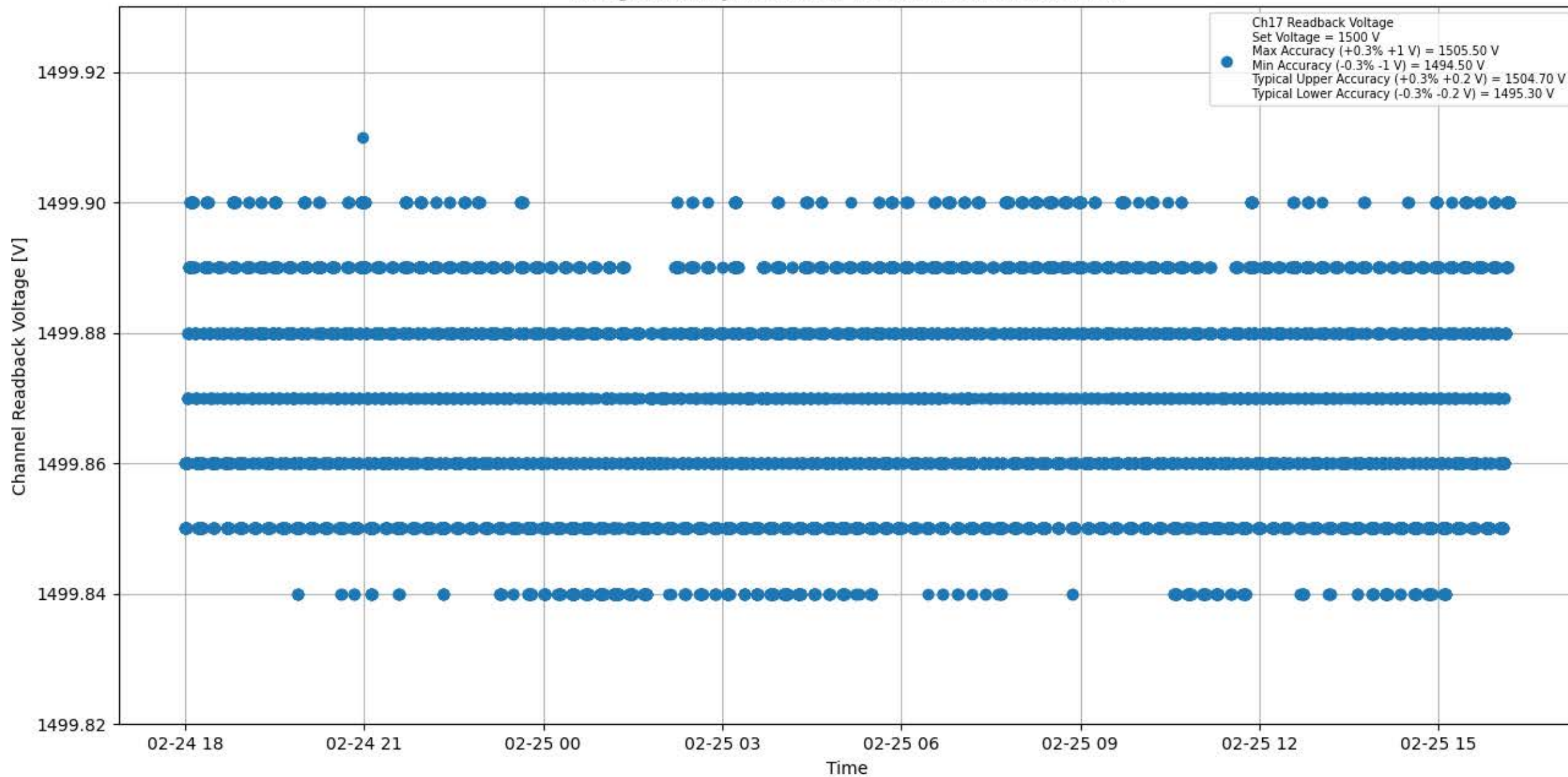
Voltage Stability 1500 V for Module #094 Channel #17
