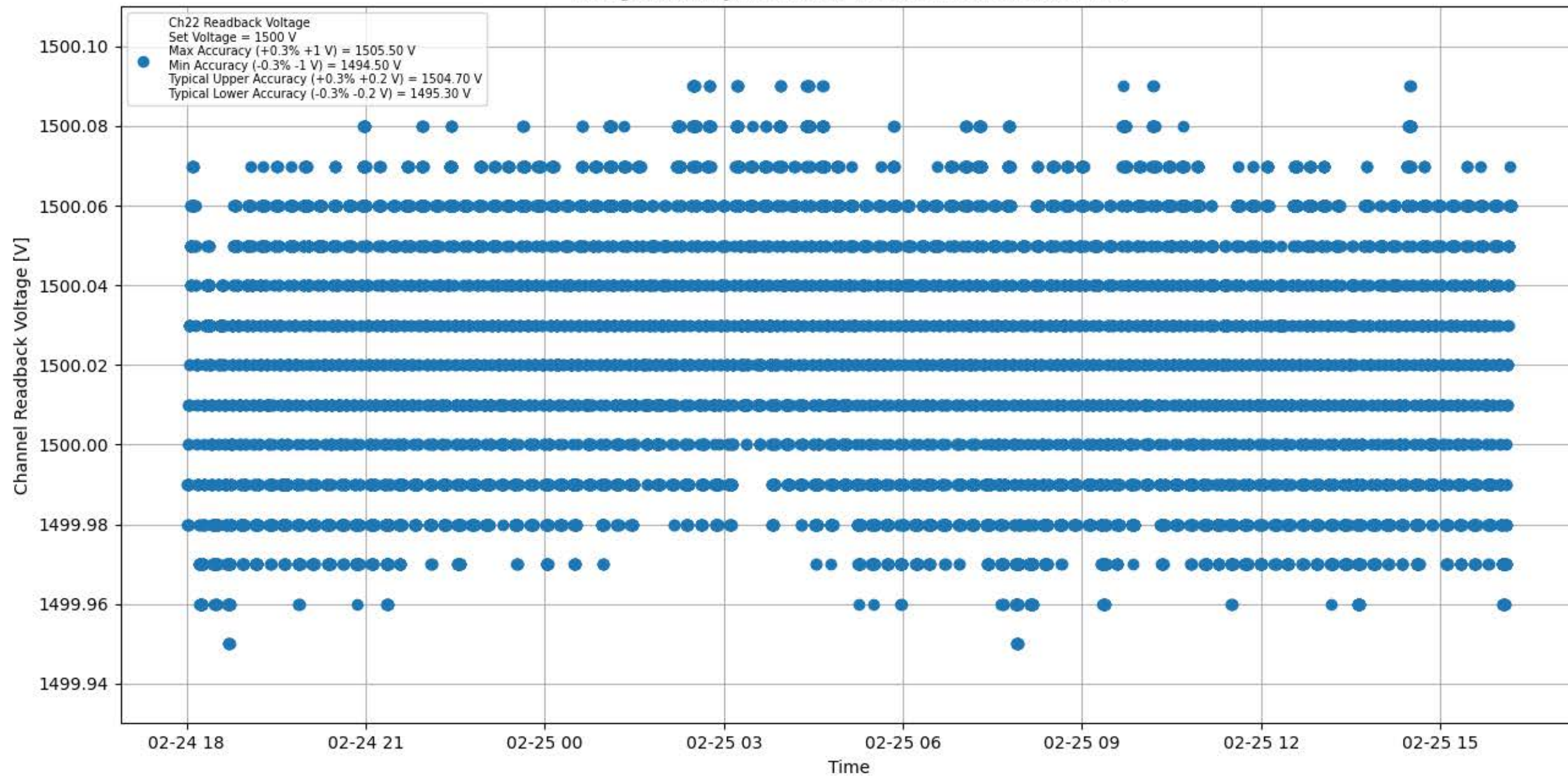
Voltage Stability 1500 V for Module #094 Channel #22
