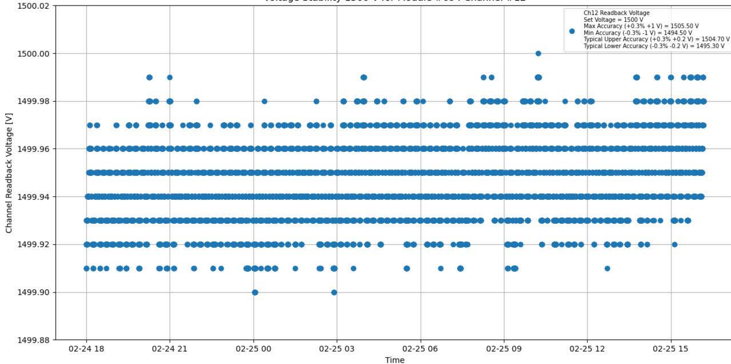
Voltage Stability 1500 V for Module #094 Channel #12
