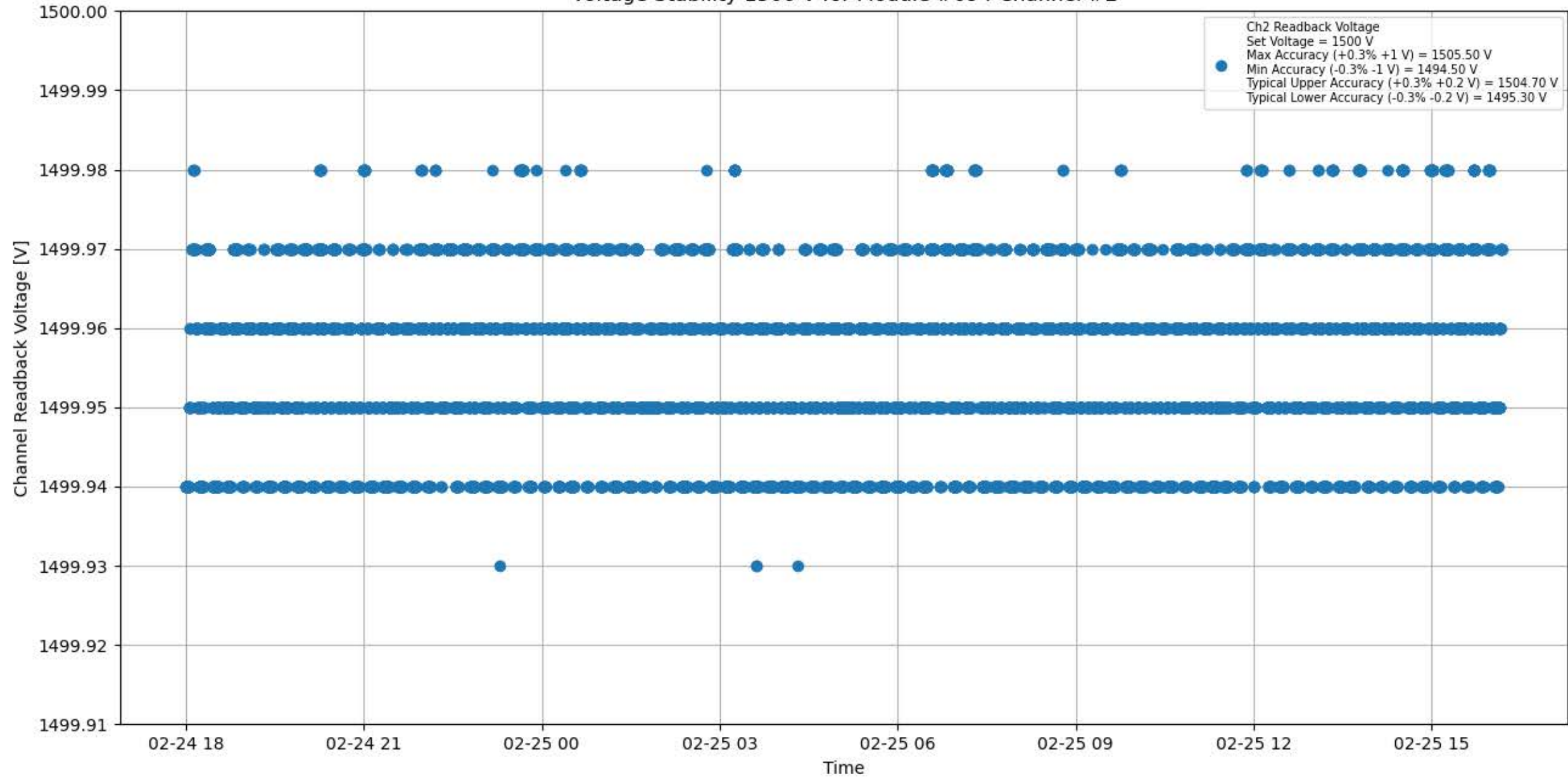
Voltage Stability 1500 V for Module #094 Channel #2
