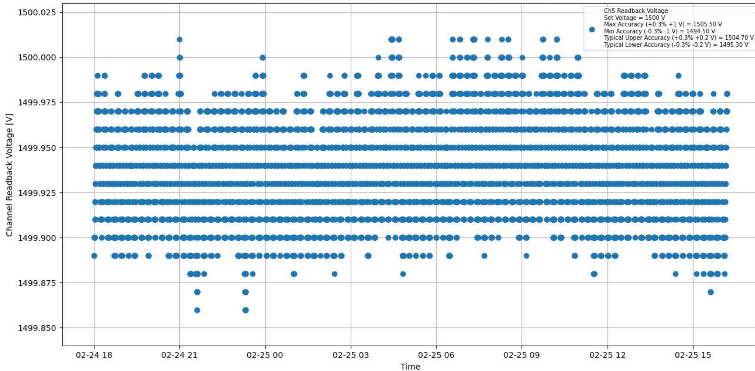
Voltage Stability 1500 V for Module #094 Channel #5
