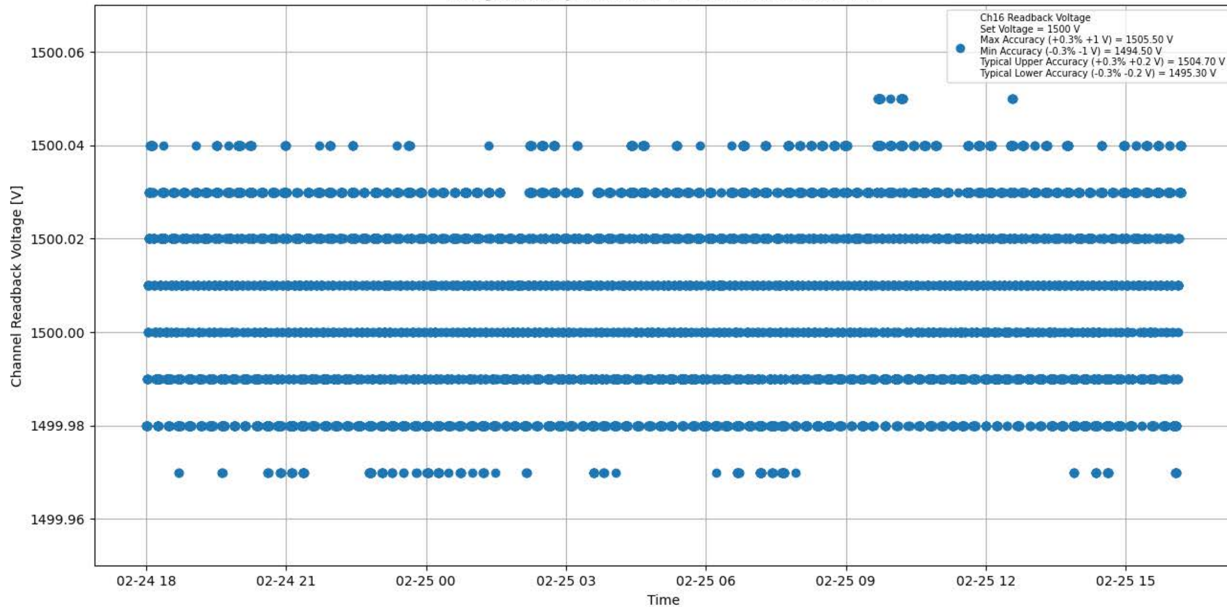
Voltage Stability 1500 V for Module #094 Channel #16
