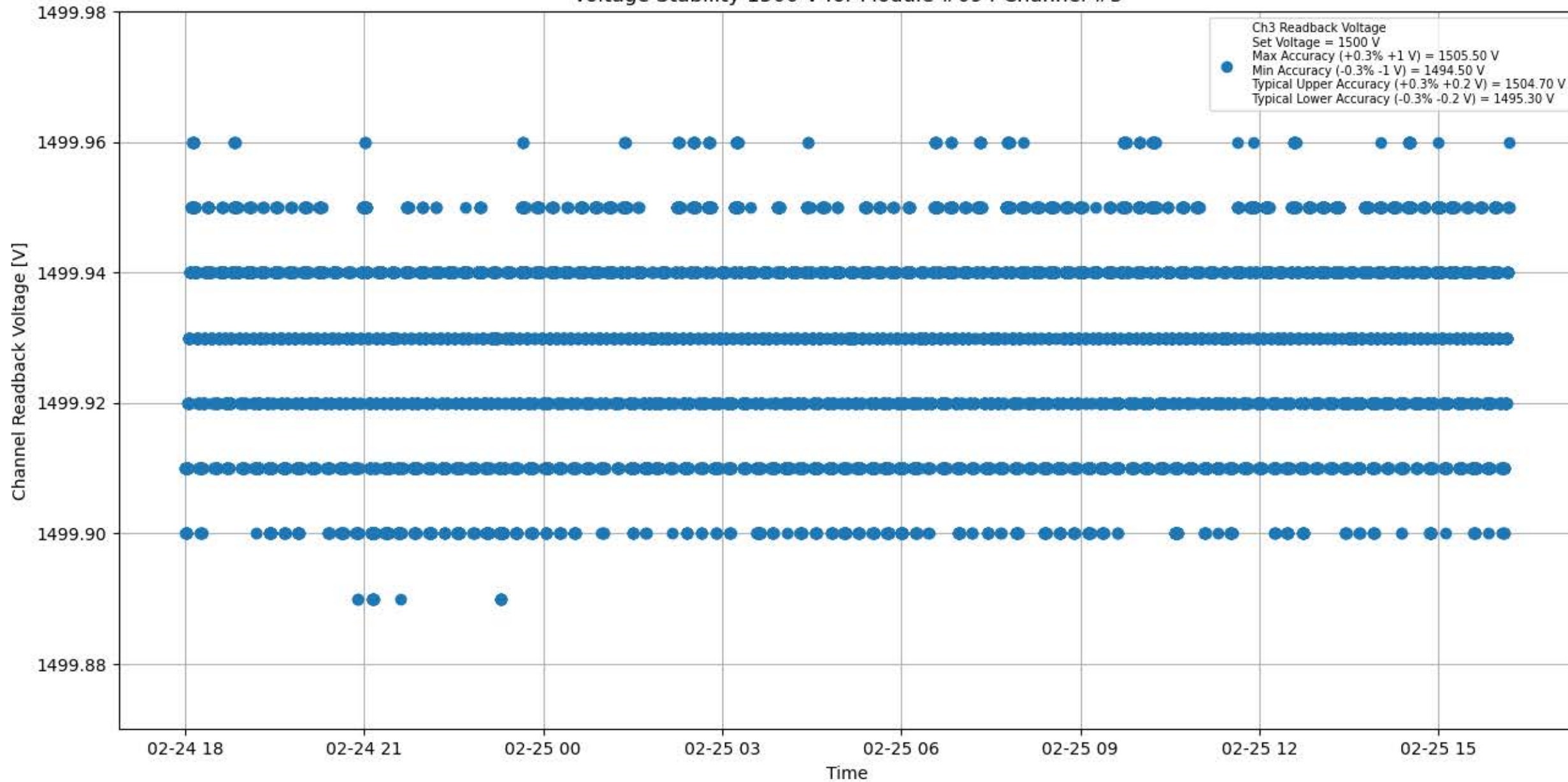
Voltage Stability 1500 V for Module #094 Channel #3
